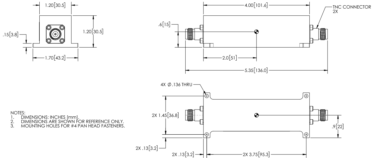
Figure B-2 GRA 5500/55 External Filter Outline Drawing (011-06280-00)
