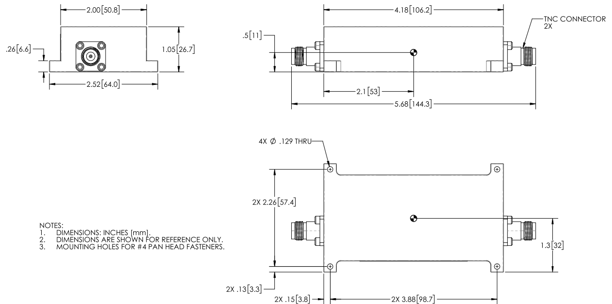
Figure B-3 GRA 5500/55 External Filter Outline Drawing (011-06280-10)
